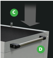
Vertical peg panel can be retracted and locked into the cabinet.
